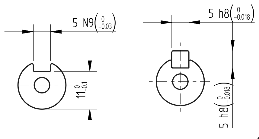
Dimension of shaft end Dimension of shaft end with key
