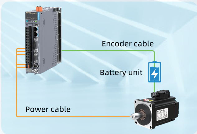
Encoder with battery
