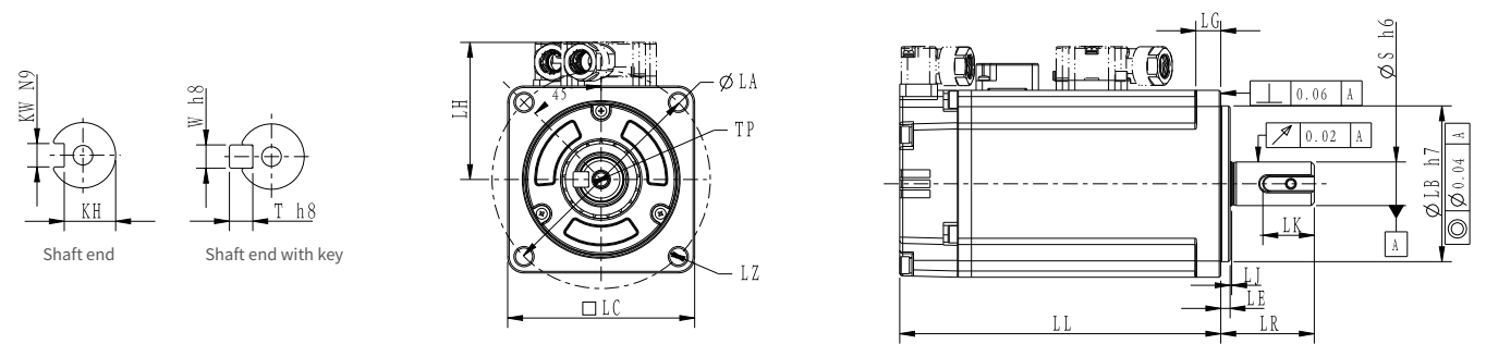
Flange size 60/80
